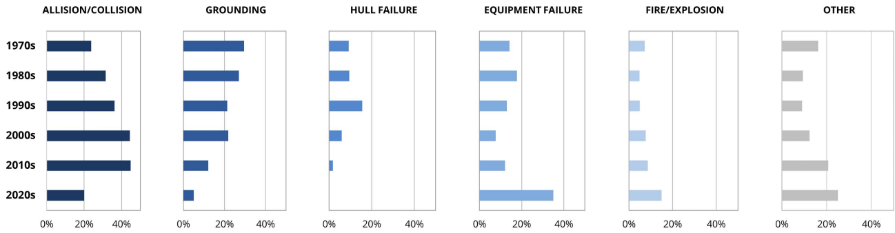
FIGURE 10: CAUSES OF TANKER SPILLS PER DECADE, 1970-2023
