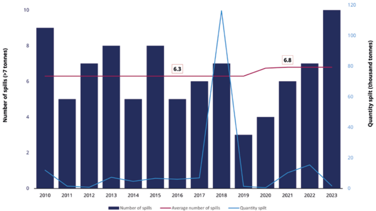
FIGURE 15: NUMBER OF TANKER SPILLS AND QUANTITIES OF OIL SPILT (>7 TONNES) FROM 2010-2023
